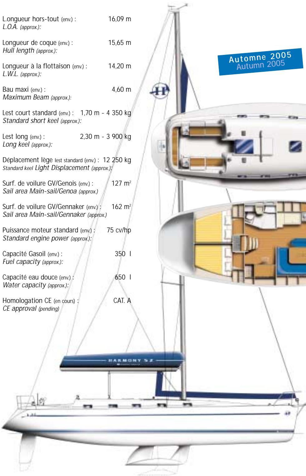
Version 3 cabines / 3 cabins version
